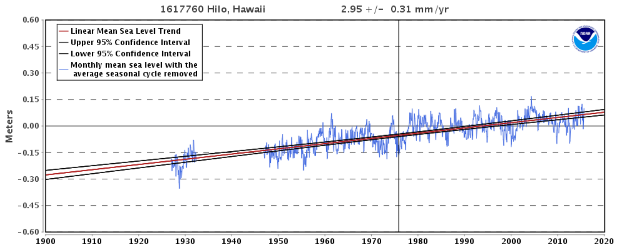
Figure 6. Observed mean-sea-level trends in the Hawaiian Islands [11]
