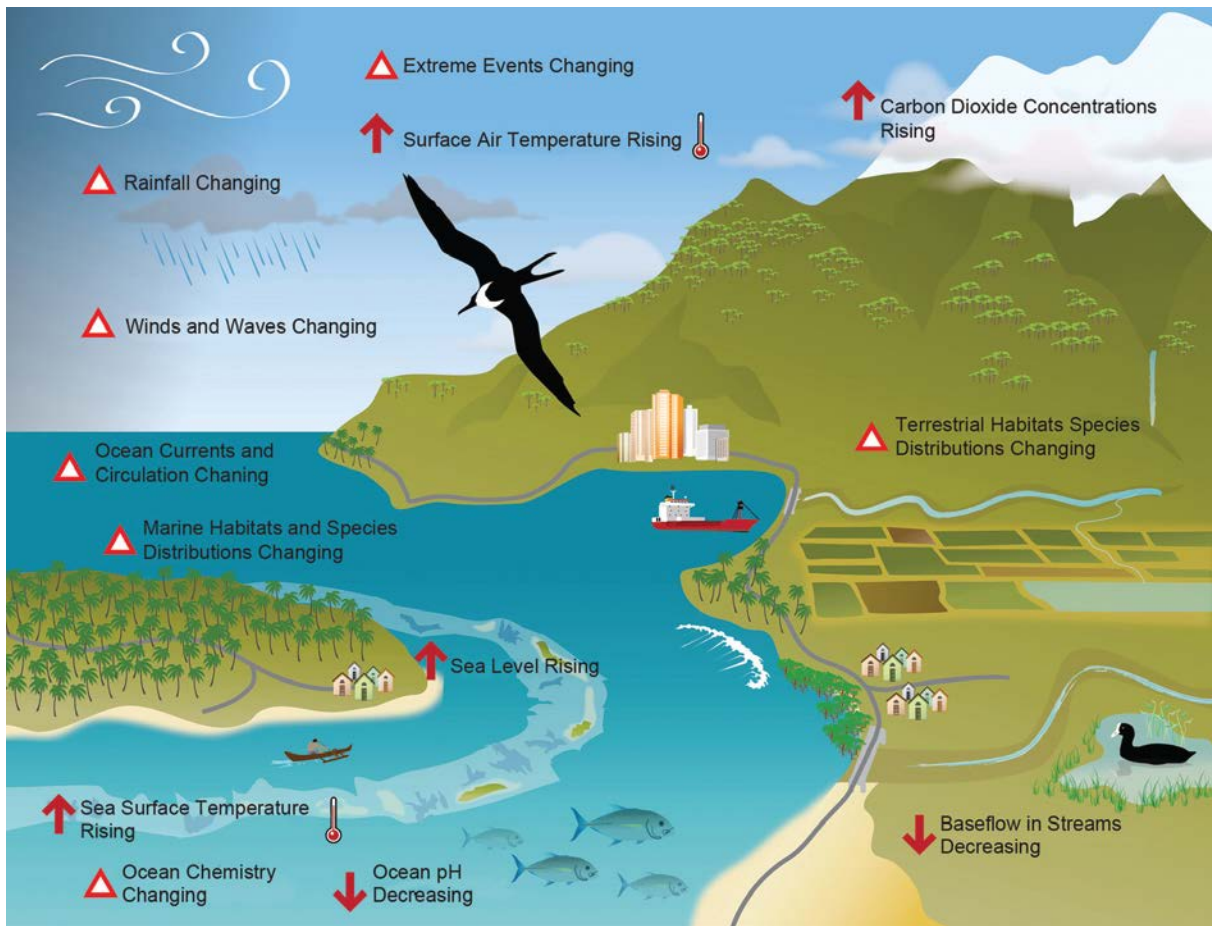
Figure 1. Indicators of climate change in the Pacific Islands region (adapted from [3])
