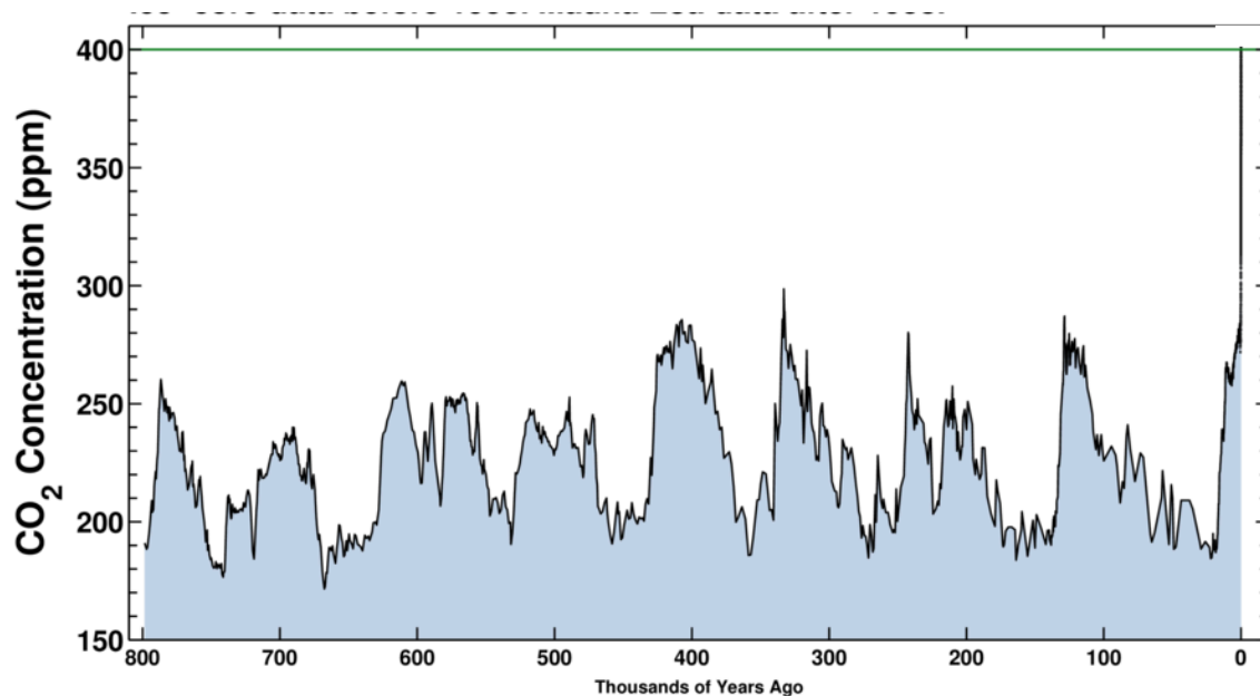
Figure 3. Current carbon dioxide concentrations in Earth's atmosphere have vastly exceeded levels measured in ice cores over the last 800,000 years [4]. Data before 1958 is from ice cores and data after 1958 are measurements taken from the Mauna Loa Observatory. Green line marks concentration of 398.02 ppm measured on October 11, 2015.
