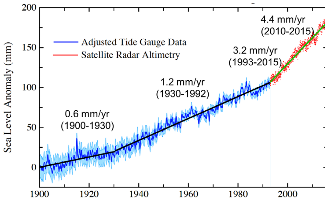
Figure 4. The observed rate of global mean sea level rise is accelerating [6-10]
