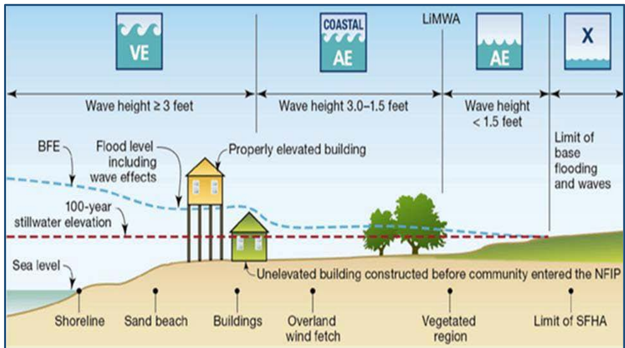
Figure 10. Coastal hazards incorporated into coastal Special Flood Hazard Zones on FEMA's Flood Insurance Rate Maps.
