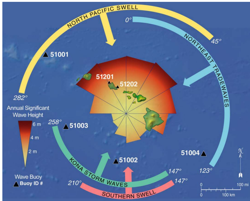
Figure 9. Dominant swell regimes and wave-monitoring buoy locations in Hawai'i [16]
