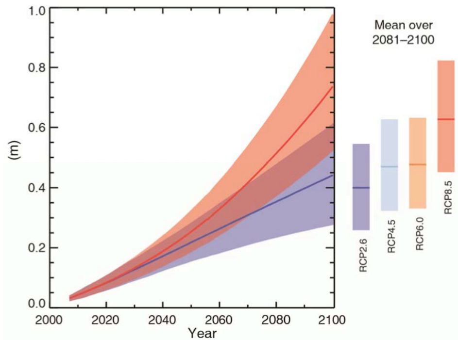
Figure 5. Projected rate of global mean sea level rise under different greenhouse gas emissions scenarios [5]. The projected rate of global sea level rise, based on the IPCC RCP 8.5 scenario, ranges from 1.6 feet (0.5 m) to 3.2 feet (0.98 m) by 2100 [4]. Recent evidence suggests that this high end scenario is the likely scenario because ice sheets and glaciers are melting at rates greater than accounted for in the IPCC report [2]
